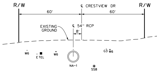
SECTION AT STA 4+50 TYPICAL FROM STA 3+21 TO 6+25
