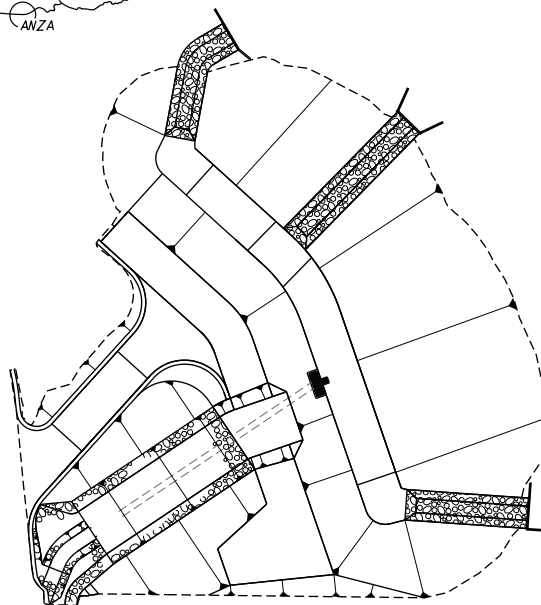
NORCO MDP LINE NA-1 DEBRIS BASIN
